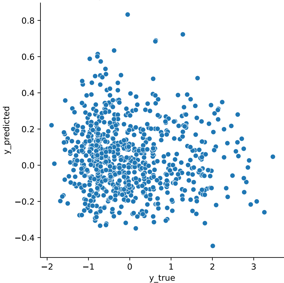
Negative affect, Random Forest
