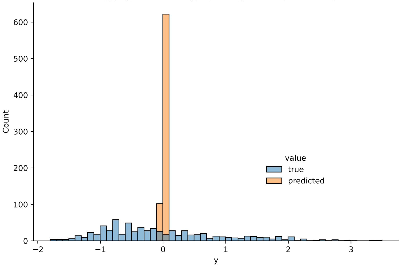
daily_24_hours,PANAS_negative_affect,Bayesian Ridge
