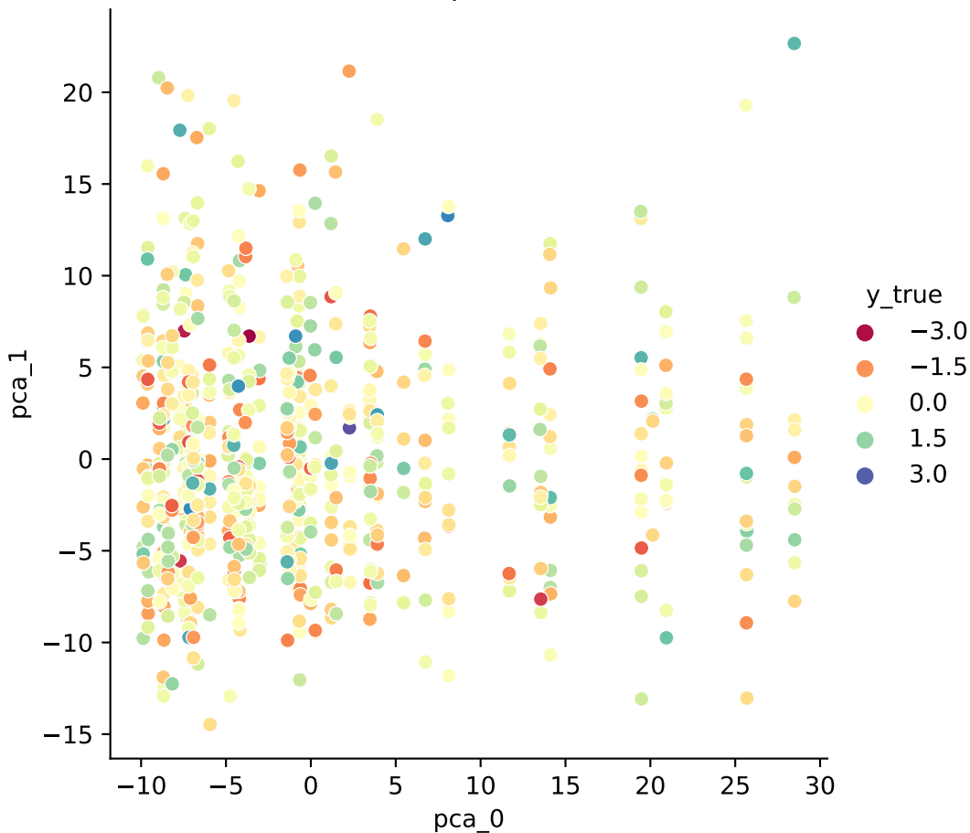
daily_24_hours,JCQ_job_demand,Bayesian Ridge variance explained = 0.29
