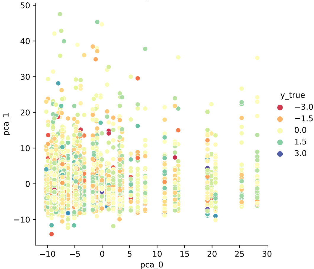
intradaily_30_min,JCQ_job_demand,Bayesian Ridge variance explained = 0.34
